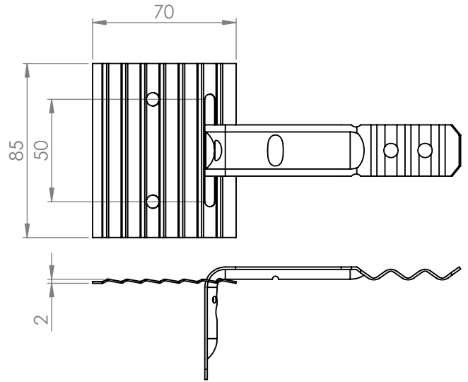
Medium duty shown - sliding bracket interchangeable
